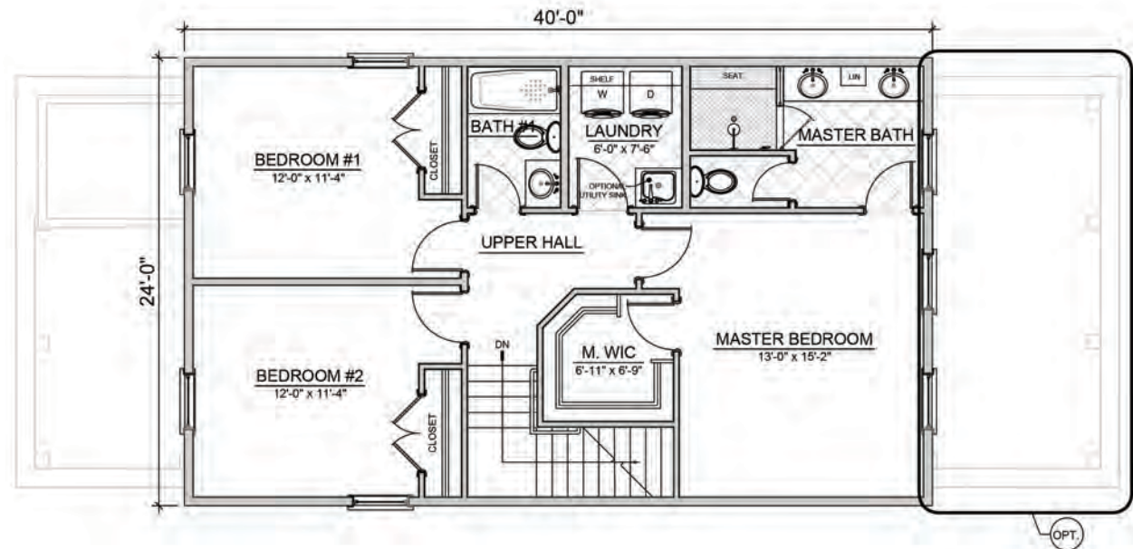
SECOND FLOOR
